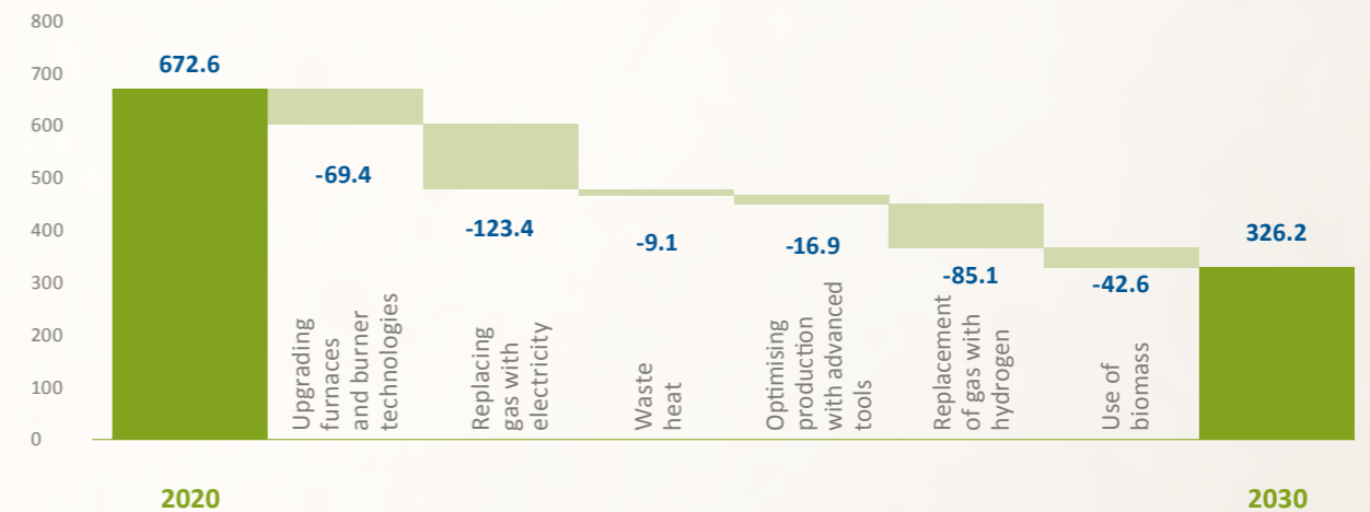
Reduction of CO 2 intensity of the company SIJ Metal Ravne (kg CO 2 /t crude steel)
