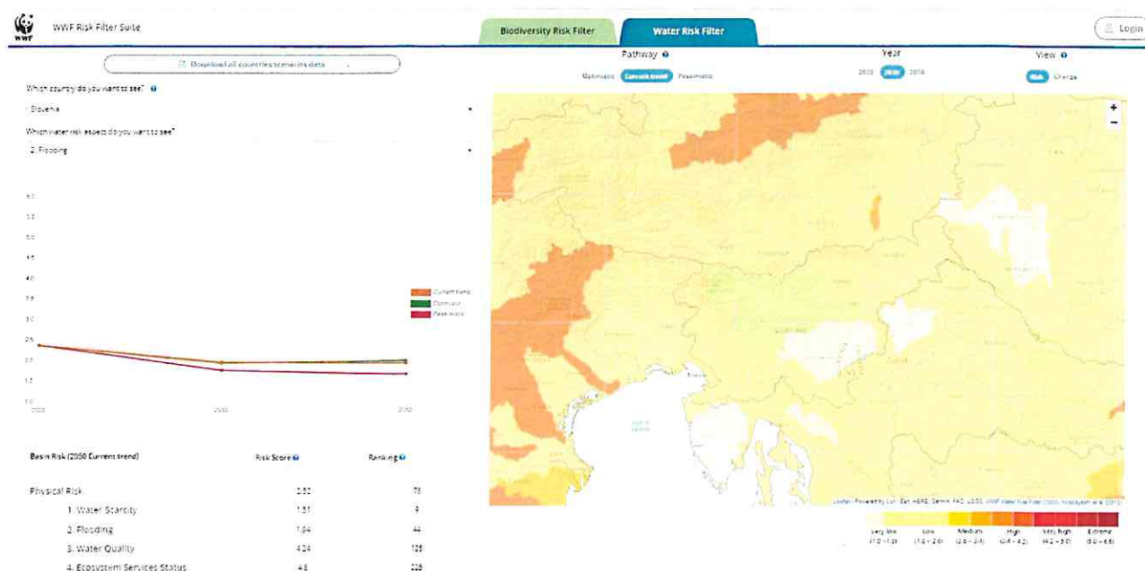
Slika 15: Scenarij poplav, vir: WWF Water Risk Filter
