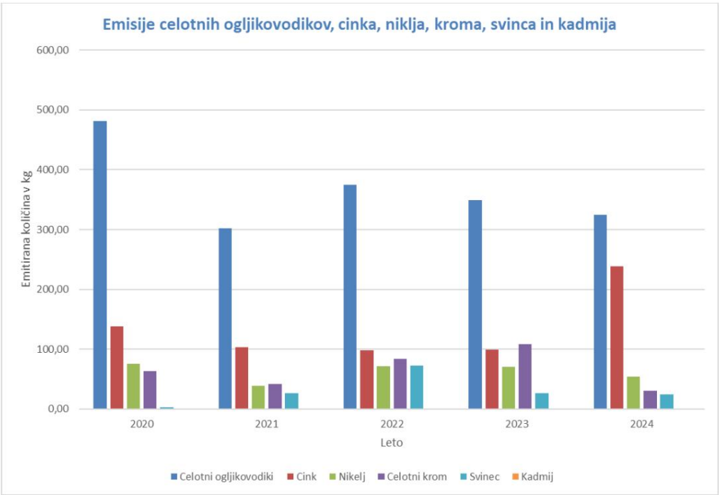
Figure 16: Emissions of total hydrocarbons, zinc, nickel, chromium, lead and cadmium (Source: Report on operational wastewater monitoring for the company SIJ Metal Ravne doo, for 2023 and 2024)
