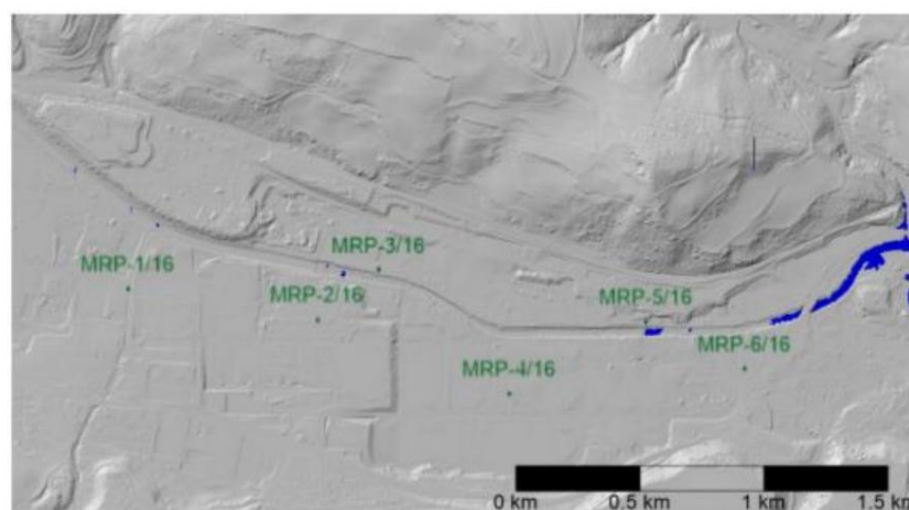
Figure 5: Display of the area of groundwater exfiltration into the Meža riverbed (measurement 20.06.2022) (Source: Baseline report for SIJ Metal Ravne doo, June 2022)
