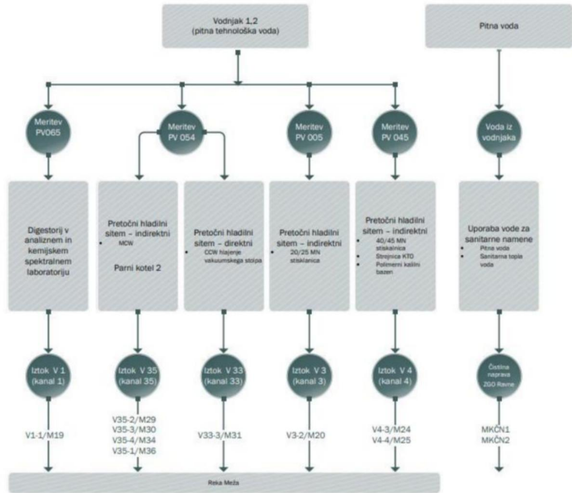
Figure 7: Scheme of potable process water outflows (Source: Report on operational wastewater monitoring for the company SIJ Metal Ravne doo, for 2022)
